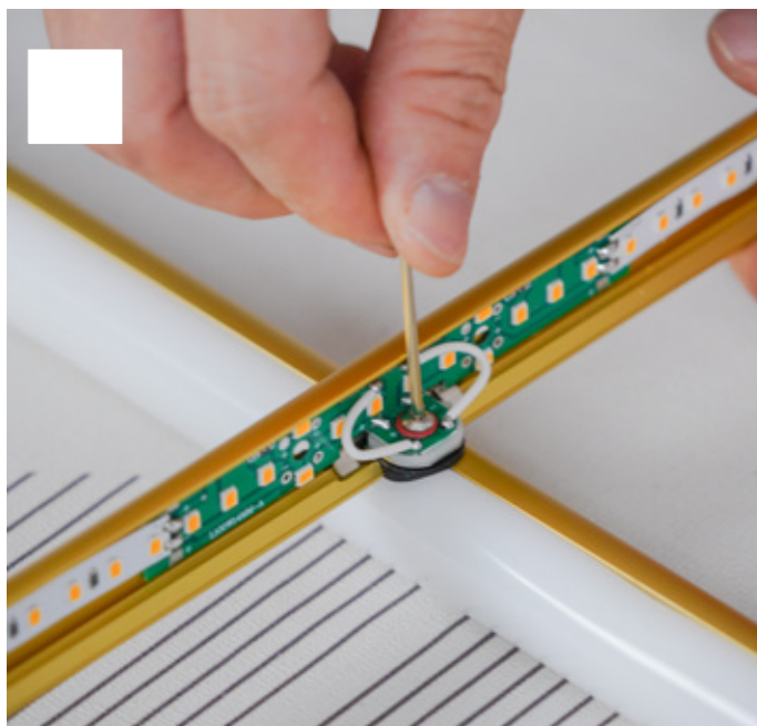
Fasten with nuts
