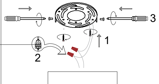
Enlarged Detail
