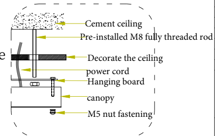
Ceiling installation diagram
