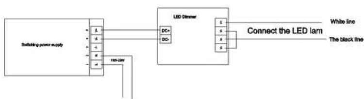
Dimmer wiring diagram
