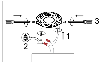
Enlarged Detail
